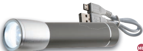
ENERGY 34913
